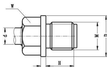
固定螺纹 Fixed screw thread
